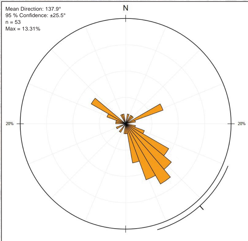
FIGURE 6 – Rose diagram of the frequency of magnetic lineaments traced in Zone 3.
