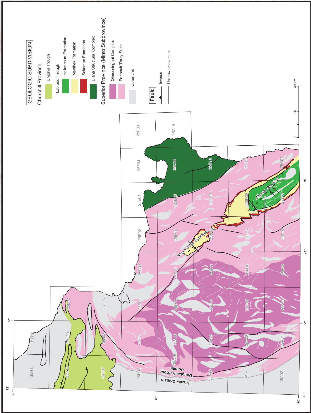
FIGURE 2B – Map of lithodemic units in the study area.
