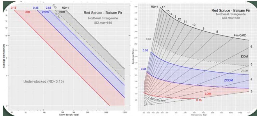
Figure 1. Updated quantitative silviculture tools for the spruce – fir forest type in the Northeast includes a stocking guide based on stand density index (SDI). This guide shows basal area ( \text{ft}^2/\text{acre} ) on the y-axis and average stand diameter (QMD) isolines (3-17 inches). It uses relative density (RD), a function of maximum and observed SDI, to define upper and lower bounds of five management zones: zone of high density-dependent mortality (DDM) (RD 1.0 - 0.67), zone of imminent competition mortality corresponding to the average self-thinning trajectory (ZICM) (RD 0.67 - 0.55); zone of optimal density management where net stand level production is expected to be highest (ZODM) (RD 0.55 - 0.35), and zone of low density management where growth rates of individual trees are optimized (LDM) (RD 0.35 - 0.15). RD < 0.15 is considered understocked relative to wood production objectives. This figure compares the updated guide (black lines) to previous spruce – fir stocking guides published by the U.S. Forest Service (Solomon et al. 1987 in orange, and Frank and Bjorkbom 1973 in green). The data points shown are from the U.S. Forest Service, FIA (colored dots) and the CFRU Commercial Thinning Research Network (black solid dots = unthinned, black hollow dots = thinned). Many of the data points fall outside the bounds of previously published stocking guides; the new guide more accurately reflects spruce – fir forest dynamics. The choice of \text{SDI}_{\text{max}}=580 corresponds to average values for red spruce and balsam fir used to predict density-dependent mortality in the Northeast Variant of the Forest Vegetation Simulator; other values can be used. Credit: David Ray. Graph is available with additional explanation in the Supplementary Materials of Ray et al. 2023 .
