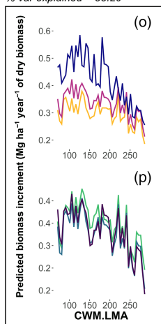
FIGURE 3 Predicted biomass increment ( \text{Mg ha}^{-1} \text{ year}^{-1} of dry biomass) as a function of important diversity features for net forest productivity, survivor growth, recruitment and mortality, with variations in mean or maximum annual temperature ( ^{\circ}\text{C} ) and minimum total annual precipitation (mm) calculated based on observed data range. Important diversity features are as follows: the community-weighted means of leaf mass per area (CWM.LMA), seed frequency (CWM.SeFreq) and drought tolerance (CWM.TolD), the functional dispersion index based on leaf traits (FDis.Leaf; i.e. leaf size, leaf longevity, leaf mass per area, and nitrogen content per leaf mass unit), the functional dispersion index based only on the leaf nitrogen content trait (FDis.Nmass), the functional dispersion index based on three traits (FDis.3, i.e. ectomycorrhiza, wood decay resistance and vegetative reproduction), and the functional dispersion index based on five traits (FDis.5, i.e. average maximum height, frequency of a good crop year, drought tolerance, root depth and leaf longevity). Diversity features are limited to between the 10th and 90th percentiles.
