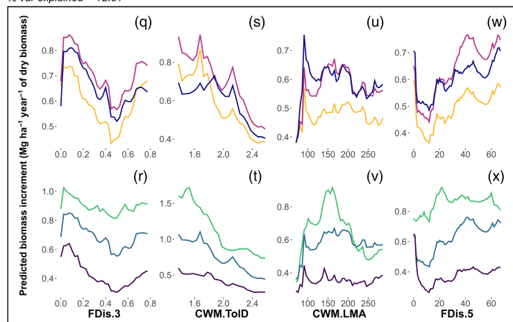
FIGURE 3 Predicted biomass increment ( \text{Mg ha}^{-1} \text{ year}^{-1} of dry biomass) as a function of important diversity features for net forest productivity, survivor growth, recruitment and mortality, with variations in mean or maximum annual temperature ( ^{\circ}\text{C} ) and minimum total annual precipitation (mm) calculated based on observed data range. Important diversity features are as follows: the community-weighted means of leaf mass per area (CWM.LMA), seed frequency (CWM.SeFreq) and drought tolerance (CWM.TolD), the functional dispersion index based on leaf traits (FDis.Leaf; i.e. leaf size, leaf longevity, leaf mass per area, and nitrogen content per leaf mass unit), the functional dispersion index based only on the leaf nitrogen content trait (FDis.Nmass), the functional dispersion index based on three traits (FDis.3, i.e. ectomycorrhiza, wood decay resistance and vegetative reproduction), and the functional dispersion index based on five traits (FDis.5, i.e. average maximum height, frequency of a good crop year, drought tolerance, root depth and leaf longevity). Diversity features are limited to between the 10th and 90th percentiles.
