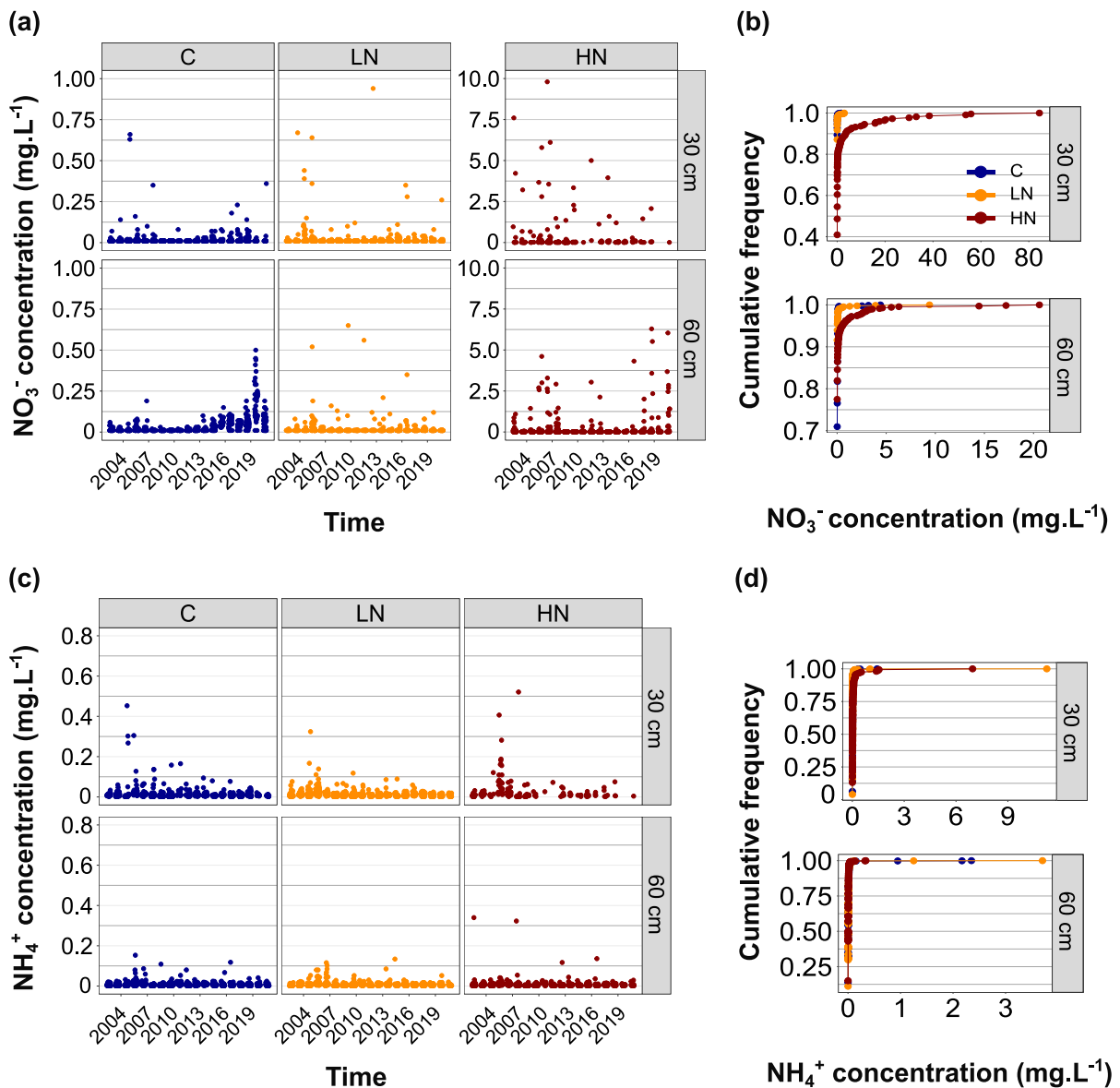
Fig. 3 Temporal variations (2002–2020) and cumulative frequencies of weekly measured soil solution \text{NO}_3^- (a, b) and \text{NH}_4^+ (c, d) concentrations at 30 and 60 cm depths at a Canadian experimental boreal forest submitted to three N treatments
